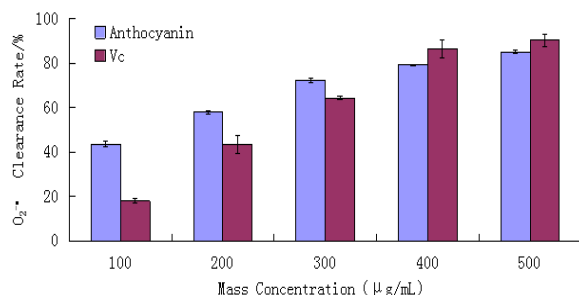
Figure 3: O 2 - scavenging activity of Aronia melanocarpa anthocyanins (AMP) and VC
